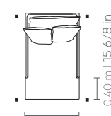
CH 2B AST ENC DEC 0,90 x 1,60 m | 35 3/8 x 63 in 1 1 2 1,00 x 1,60 m | 39 3/8 x 63 in 1 1 2 1,10 x 1,60 m | 43 2/8 x 63 in 1 1 3 1,20 x 1,60 m | 47 2/8 x 63 in 1 1 3 1,30 x 1,60 m | 51 1/8 x 63 in 1 1 3
